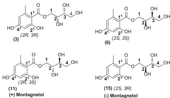
Figure 1. Montagnetol and its isomers.
