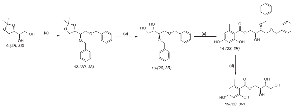
Scheme 3. Synthesis of (-) Montagnitol 15 . Reaction Condition: (a) NaH, BnBr, DMF, rt, 12 h; (b) PTSA, MeOH, rt, 1 h; (c) orsellinic acid, DCC, DMAP, THF, rt 3 h, (d) Pd/C, \text{H}_2 , EtOAc, 3 h.
