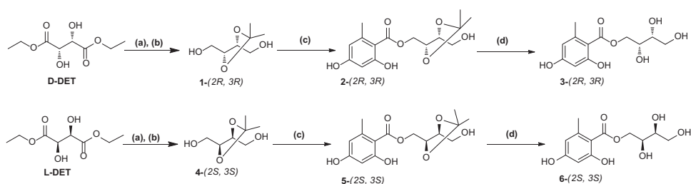
Scheme 1. Synthesis of compounds 3 and 6 . Reaction Condition: (a) 2,2-DMP, p -TsOH, dry acetone, rt, 12 h; (b) LAH, dry THF, 70 °C, 1 h; (c) DCC, DMAP, THF, rt, 3 h; (d) p -TsOH, MeOH, rt, 1 h.
