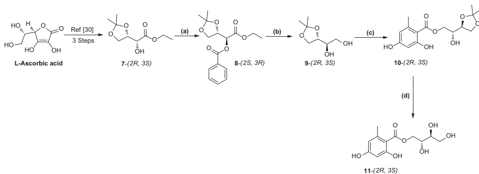
Scheme 2. Synthesis of (+) Montagnitol 11 . Reaction Condition: (a) \text{Ph}_3\text{P} , DEAD, \text{PhCOOH} , dry THF, rt, 12 h; (b) LAH, dry THF, 12 h; (c) Orsellinic acid, DCC, DMAP, THF, rt 3 h; (d) p -TsOH, MeOH, rt, 1 h.
